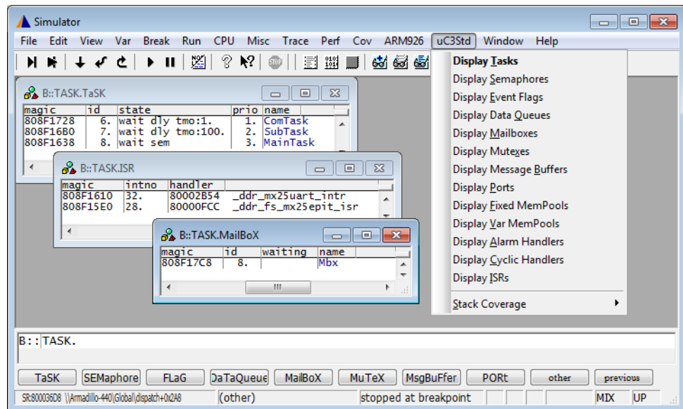
TRACE32 with \mu C3/Standard menu
