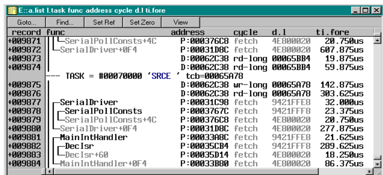
Analyzer listing, function call hierarchy and task switches
