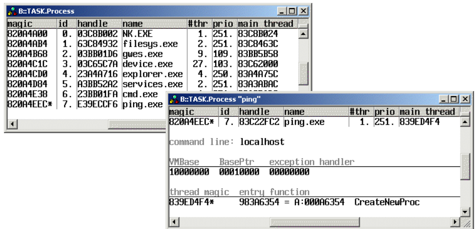
Process list and detailed view of one process
