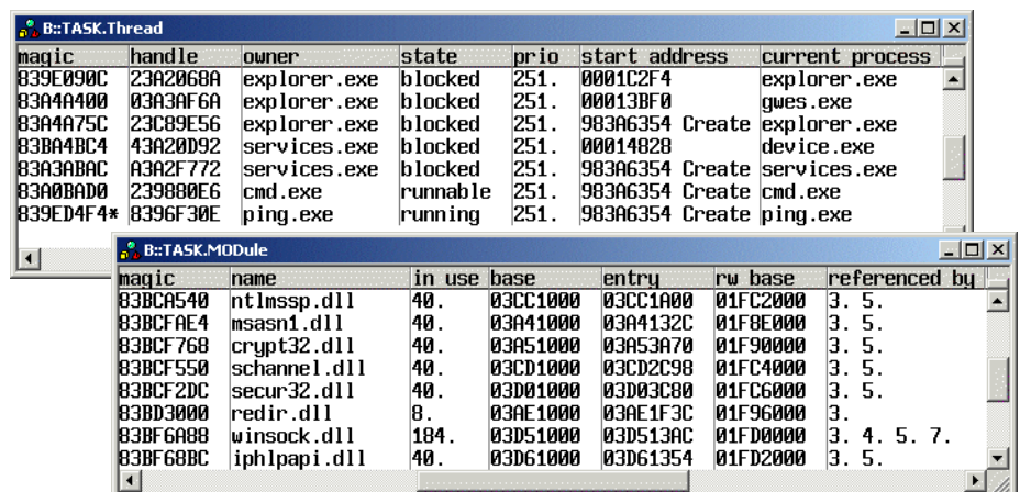
Thread list and DLL list window
